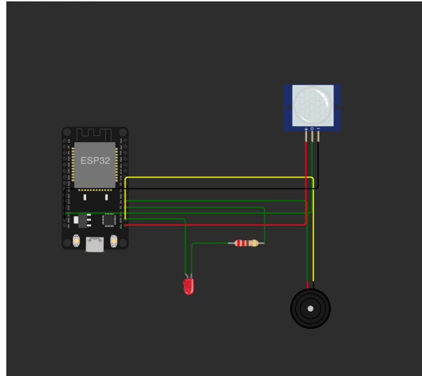
Figure 2: Wokwi Circuit Diagram of Smart Intrusion Detection System
